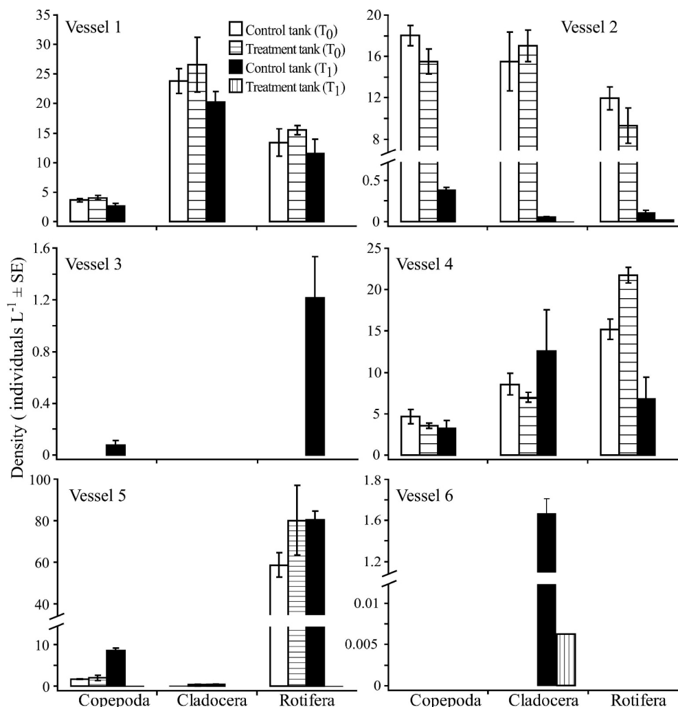
Fig. 3. (A–F) Density (individuals L^{-1} \pm standard error [SE]) of copepods, cladocerans, and rotifers sampled from treatment (exchanged) and control (not-exchanged) ballast tanks at the beginning ( T_0 ) and end ( T_1 ) of the ships' voyages. Note breaks in the y-axis for vessels 2, 5, and 6. T_0 samples were not collected for ships 3 or 6 (see Methods ).
